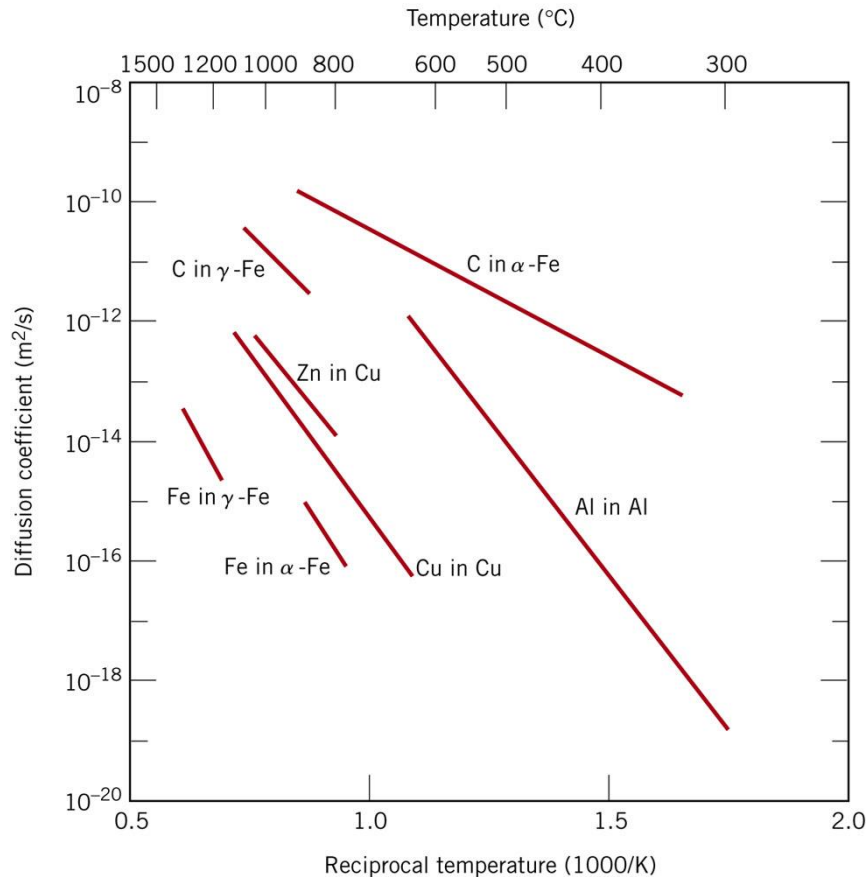
FIGURE 5.6 Plot of the logarithm of the diffusion coefficient versus the reciprocal of absolute temperature for several metals.
