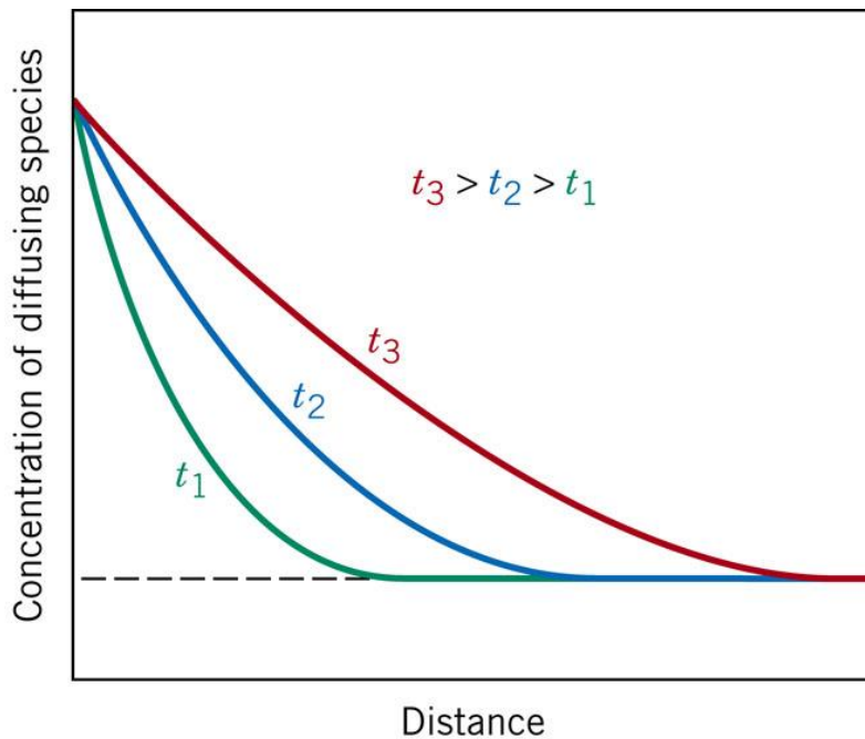
FIGURE 5. 6 Concentration profiles for nonsteady-state diffusion taken at three different times, t_1 , t_2 , and t_3 .
